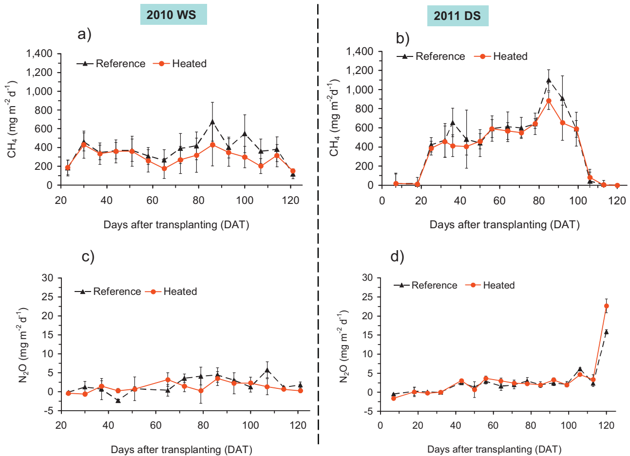
Fig. 5. Seasonal variations in ((a) and (b)) CH 4 and ((c) and (d)) N 2 O emission rates from reference and heated plots during ((a) and (c)) 2010 WS and ((b) and (d)) 2011 DS; vertical bars indicate the standard error of means ( n=4 ).
